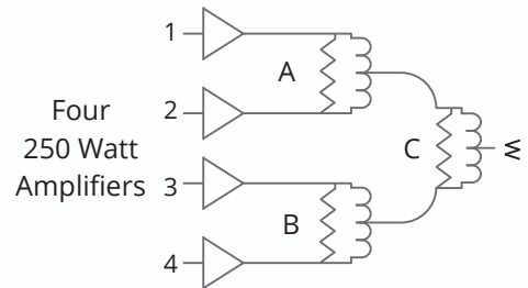
Input Failure(s) VS Power Output
