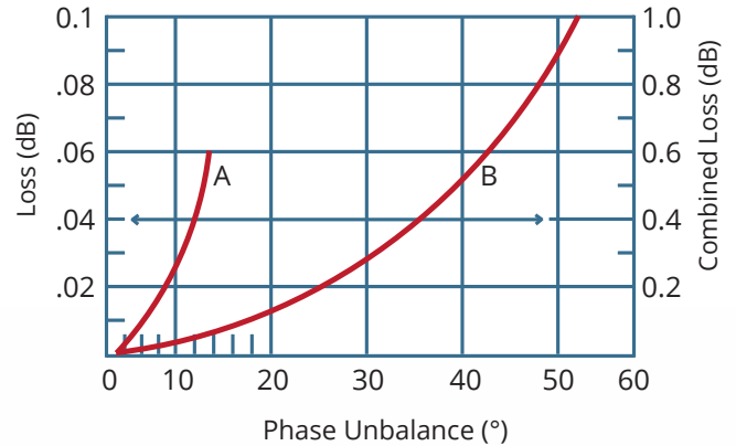
Loss VS Phase Unbalance for a Combining Hybrid w/ Equal Amplitude Inputs
