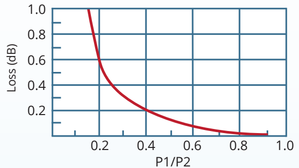
Loss VS Amplitude Unbalance for a Combining Hybrid
