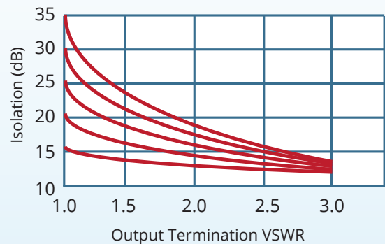
Isolation vs Output Termination VSWR for Combining Hybrid
